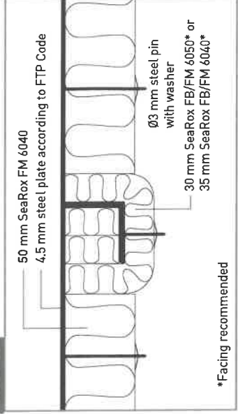
SECTION D
